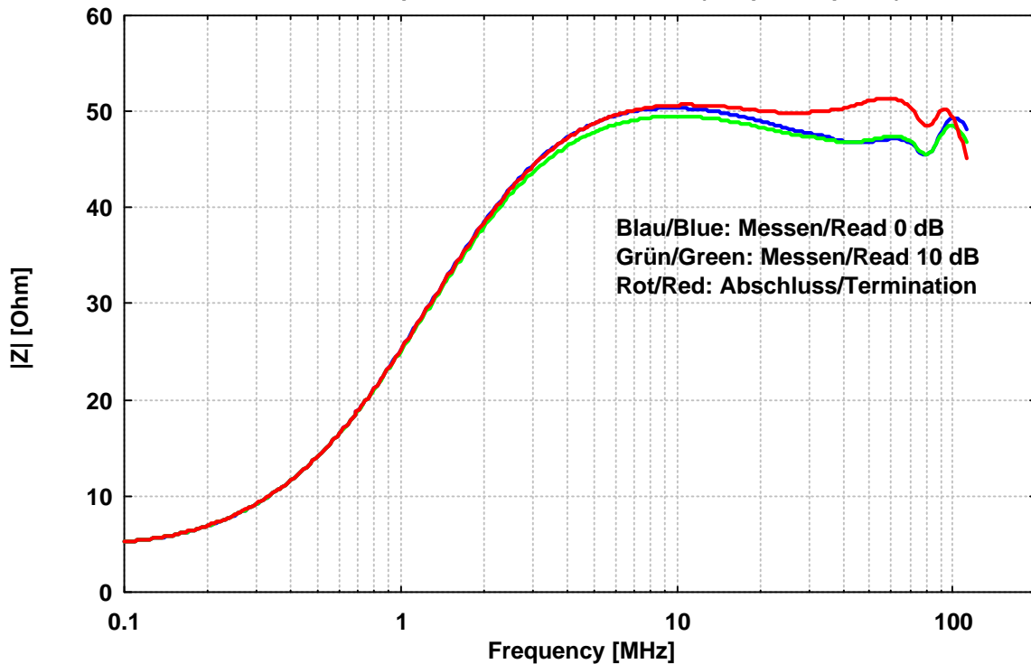
Gemessene Impedanz an den Prüflingsklemmen (Spezialadapter erforderlich) Measured Impedance at EuT-Terminals (Adapter required)
